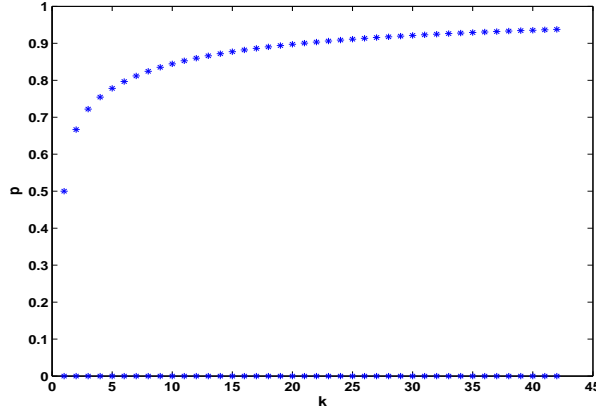
FIGURE 4. Fixed points for the ARBN model f(p) = p + \frac{1}{N}(1 - p - p^{k+1} - (1 - p)^{k+1}) . The fixed points converge to 1 as k increases.
