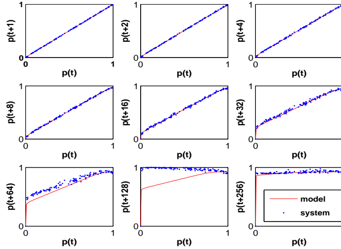
FIGURE 1. Iterations of the system and the model for ARBNs, with N = 128 and k = 32 .
