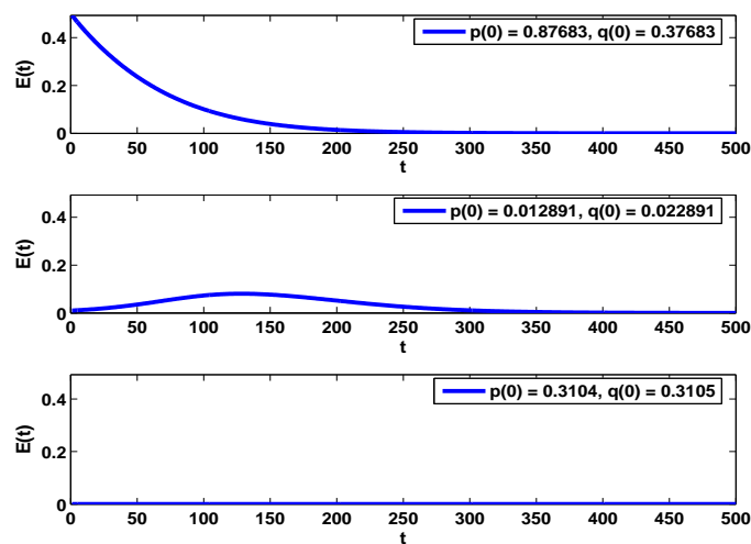
FIGURE 2. Error plot for the ARBN model with N = 128 and k = 4 . In each graph we plot the error E(t) = |p(t) - q(t)| versus t . We start with initial values p(0) and q(0) that are 0.5, 0.01, and 0.0001 apart respectively. The error converges to zero in all cases.
